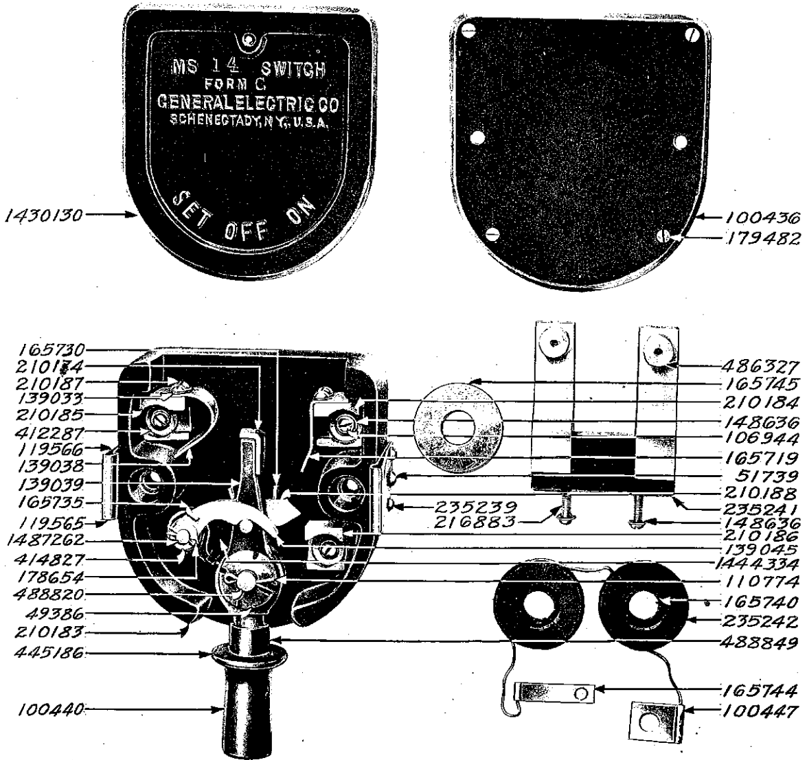
MS-14 Form G Magnetic Blowout Switch
